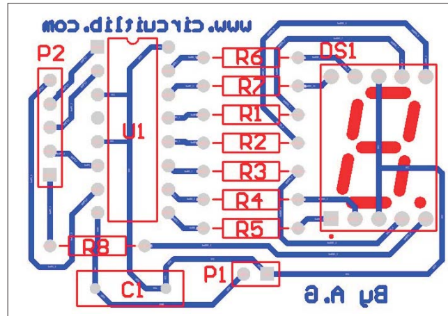
Top - View / Components Placement
