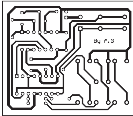
PCB layout in 1:1 scale
