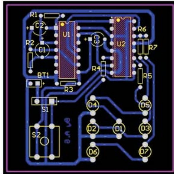
Components Placement guide - Top View
